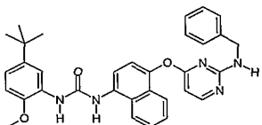
1-[4-(2-Benzylamino-pyrimidin-4-yloxy)-naphthalen-1-yl]-3-(5-tert-butyl-2-methoxy-phenyl)-urea;
